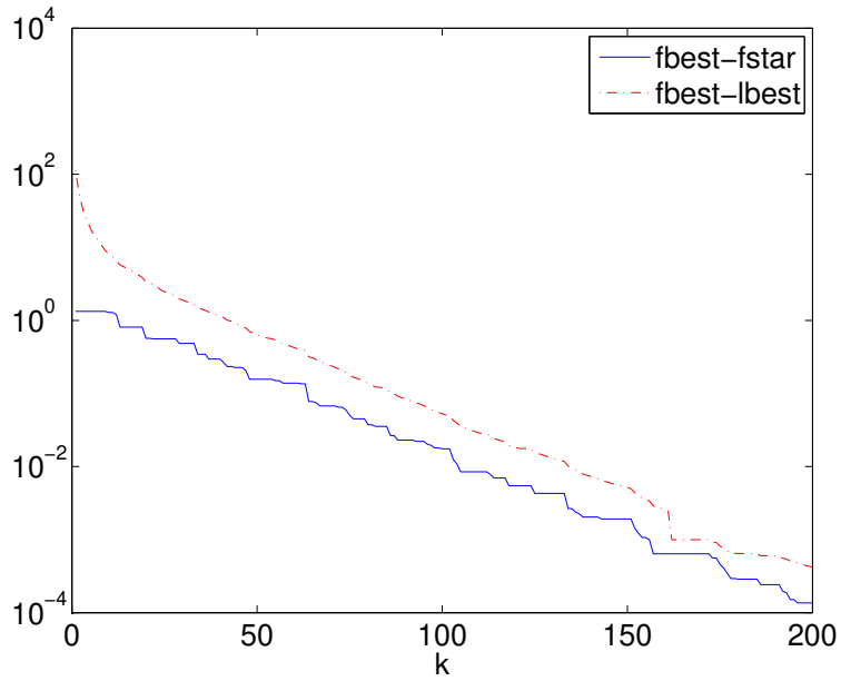
Figure 2: The value of f_{\text{best}}^{(k)} - f^* (in blue) and the value of f_{\text{best}}^{(k)} - l_{\text{best}}^{(k)} (in red) versus iteration number k for the basic ACCPM.
